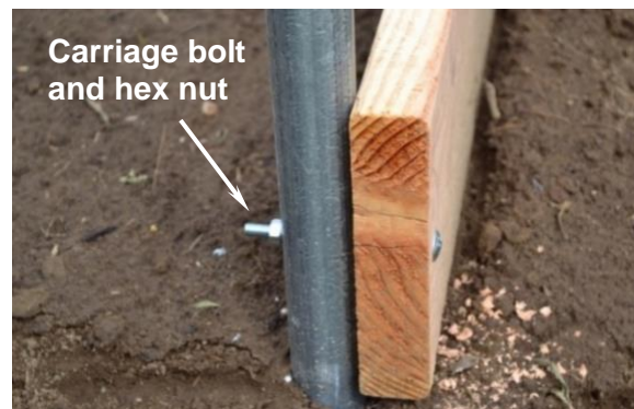
Figure 15: Attaching baseboard to the end wall.
