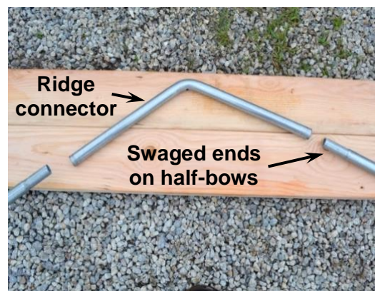
Figure 5: Bow assembly.
