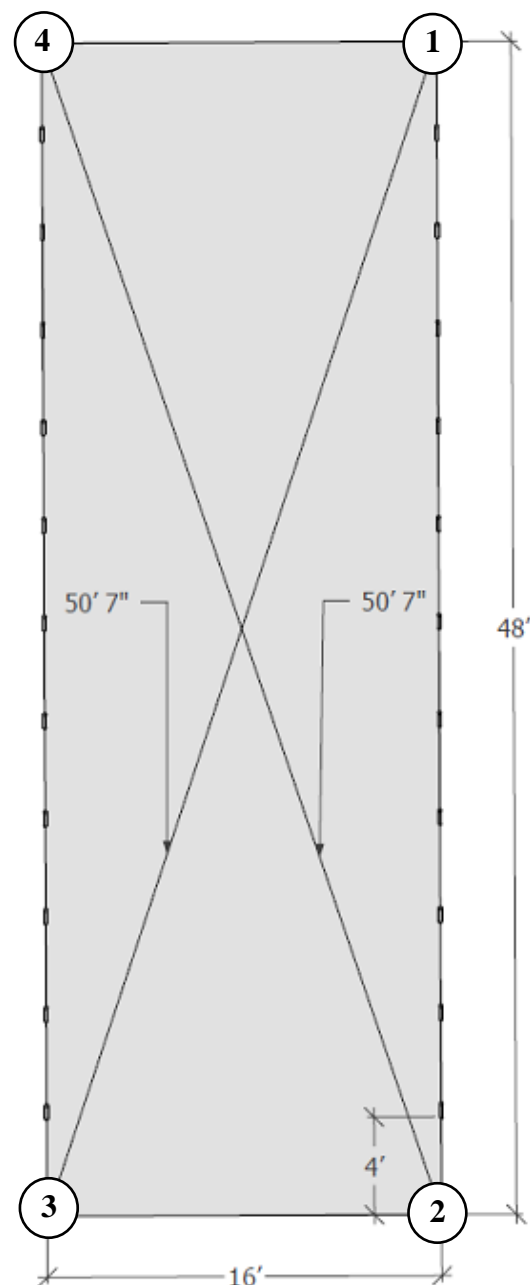
Figure 1: Diagonal measurements.
