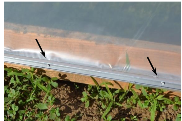
Figure 45: Tek screws securing curtain cap to the roll-up side pipe.
