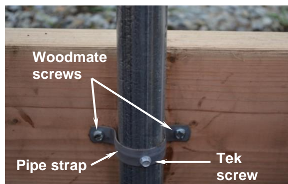
Figure 14: Attaching the baseboard to the bows.
